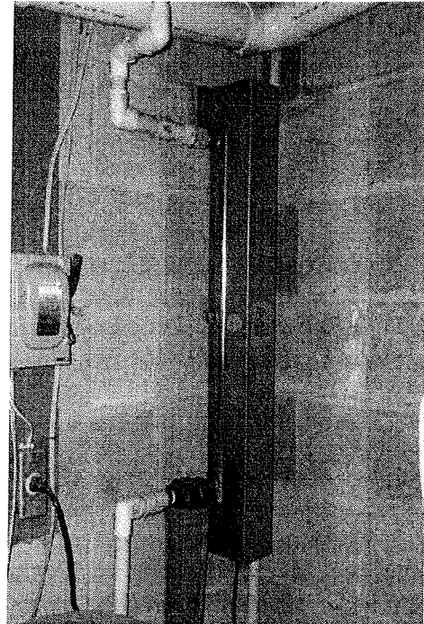
Figure 2. A typical UV light installation with a small canister sediment filter (bottom) ahead of the UV light unit.
